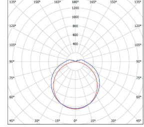
Fotometrik Veri / Photometric Data
